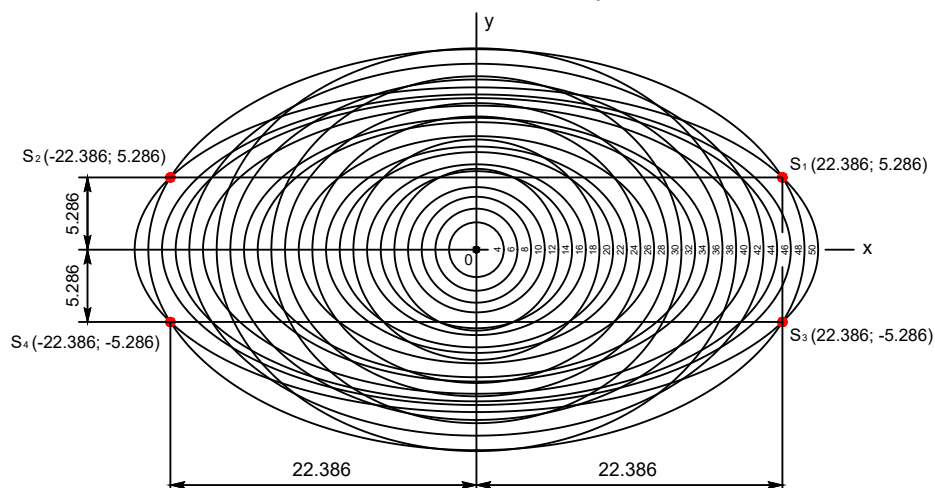
Family of ellipses of decompositions of even numbers into the sum of 2 prime numbers
