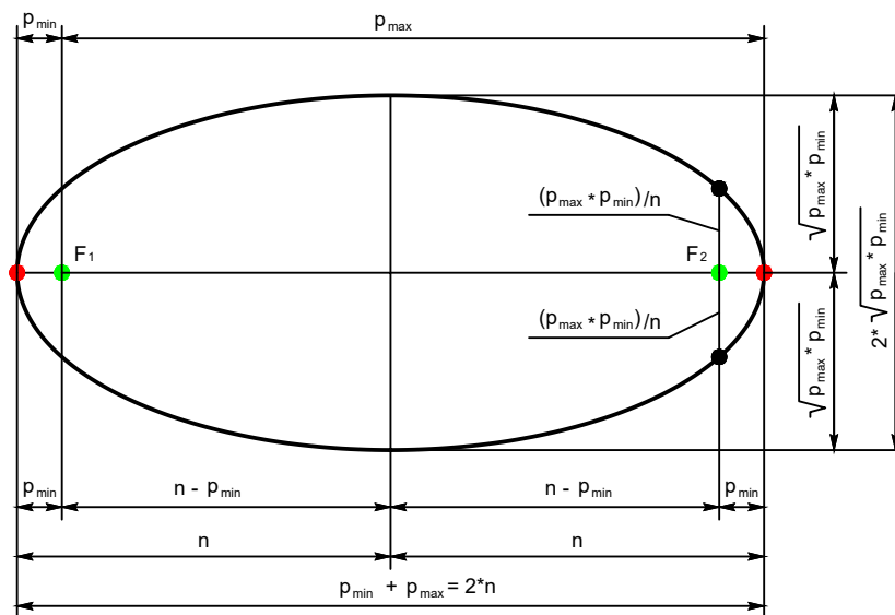
Ellipse of the decomposition of an even number into the sums of two prime numbers
