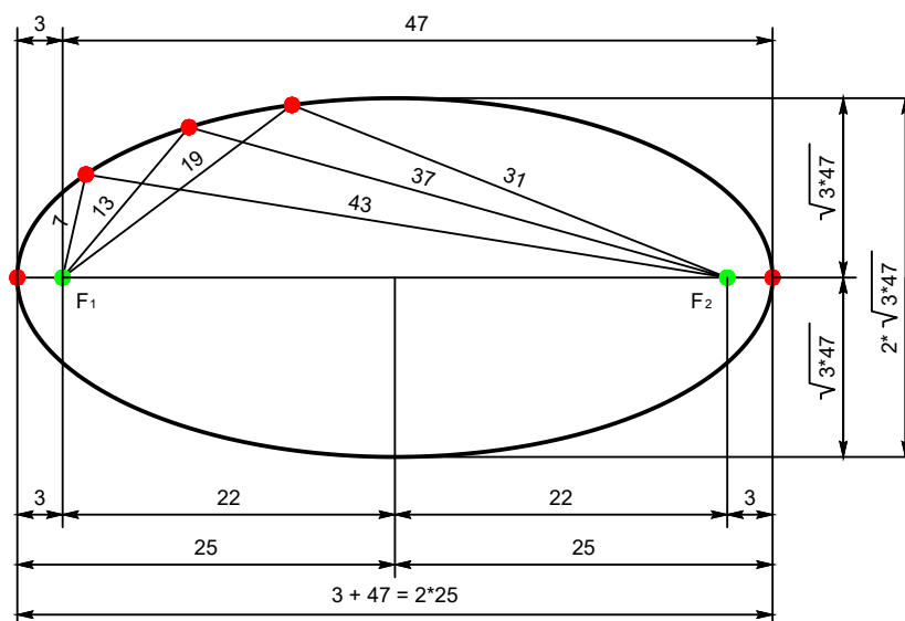
Ellipse of the decomposition of the number 50 into the sums of two prime numbers
